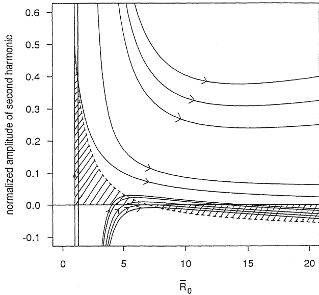
FIG. 8. Phase plane trajectories for the second harmonic ( l=2 mode) that result from perturbation by Y_{1,m} . The ordinate is the ratio of B_{2,2m}^{(2)} to the Clebsch-Gordan coefficient C_{2,2m} . The critical point is at (1, \frac{1}{2}) in these coordinates and the arrows show the direction of increasing time. \beta has been chosen to be 1.5. The broken line represents the neutral stability curve and cuts the \bar{R}_0 axis at \bar{R}_0=4+2\beta=7 . Any trajectory starting beyond this value will result in evolution into the shaded unstable region.
