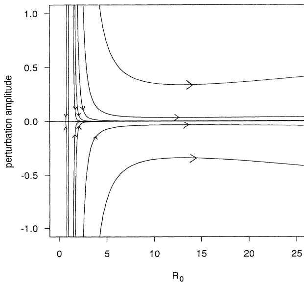
FIG. 9. Phase plane trajectories for the amplitude of the l=2 mode that result from perturbation by Y_{2,m} , shown for \beta=1.5 . The critical point is at (1,0) and the neutral stability line is the R_0 axis. Beyond R_0(1.5,2)=13 , the magnitude of the perturbation amplitude increases with R_0 and with time.
